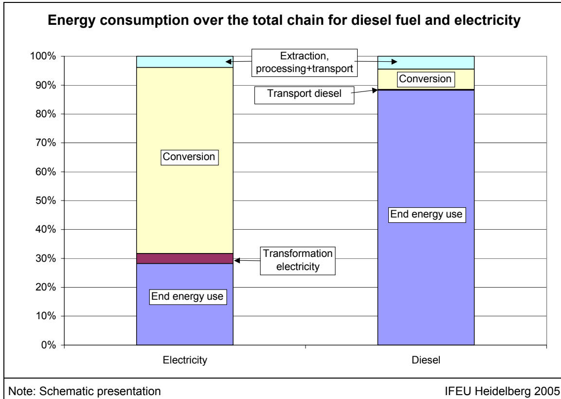
Figure 3 Energy chain for diesel fuel and electricity
