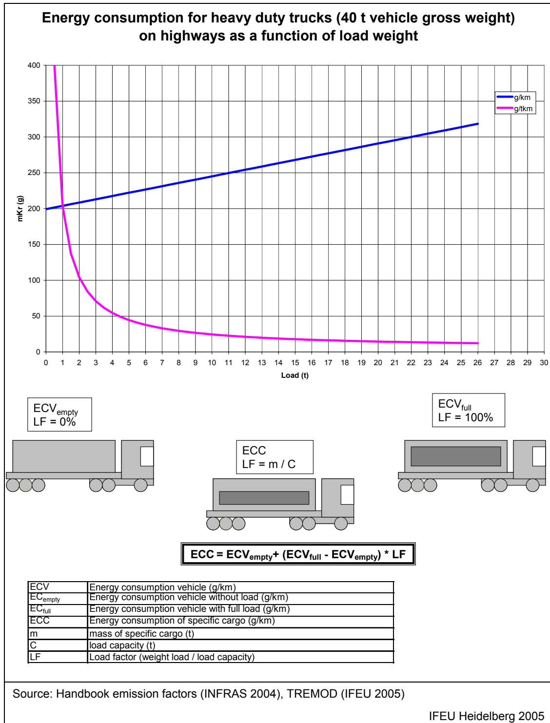
Figure 6 Example: energy consumption for heavy duty trucks (40 t vehicle gross weight) as a function of load weight
